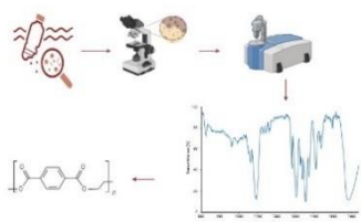
Fig.1: ATR-FTIR spectrum of MP sample showing polyethylene terephthalate (PET) Identification.
